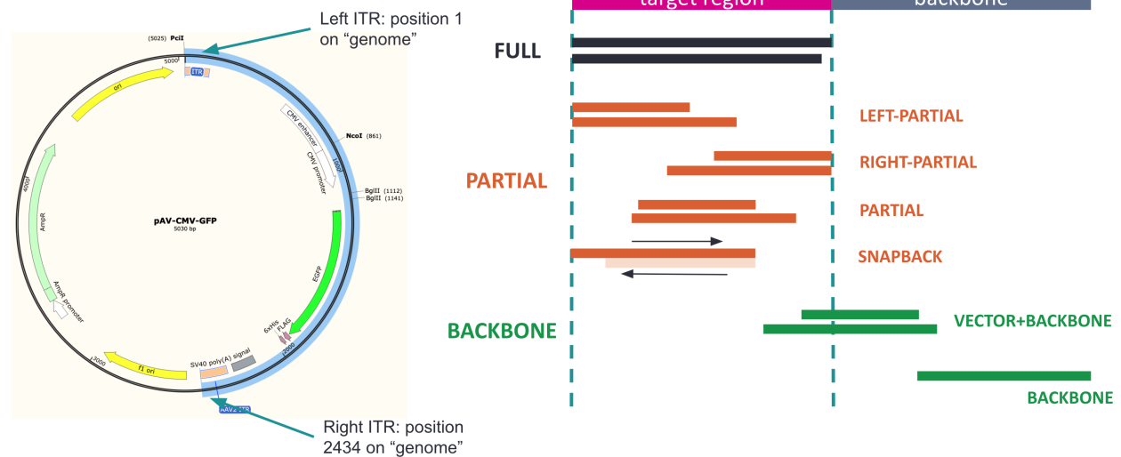
Figure 1: Single-stranded AAV types (ssAAV). ssAAV reads are expected to have a single (forward) alignment to the vector genome. “ssAAV full” reads cover the target region from left ITR to right ITR. “ssAAV left-partial” contain the left ITR but are missing the right ITR. “scAAV vector+backbone” reads overlap both the ITR-to-ITR region and the plasmid backbone, beyond the ITR.
